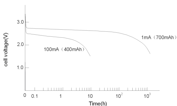
Typical 1mA, 100mA Discharge current
