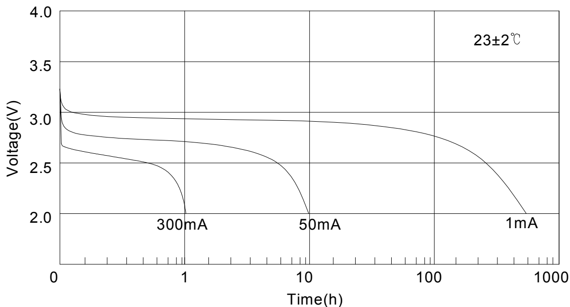
Discharge performance
