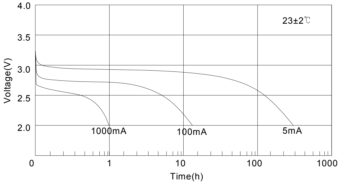
Discharge performance
