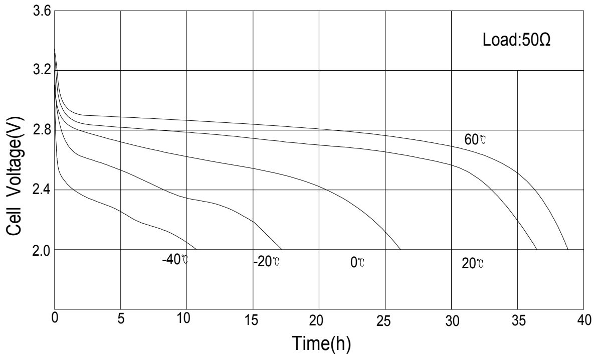
The relationship between Voltage and temperature
