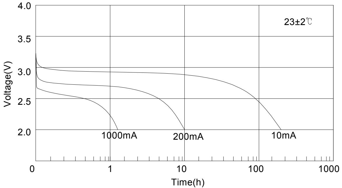
Discharge performance
