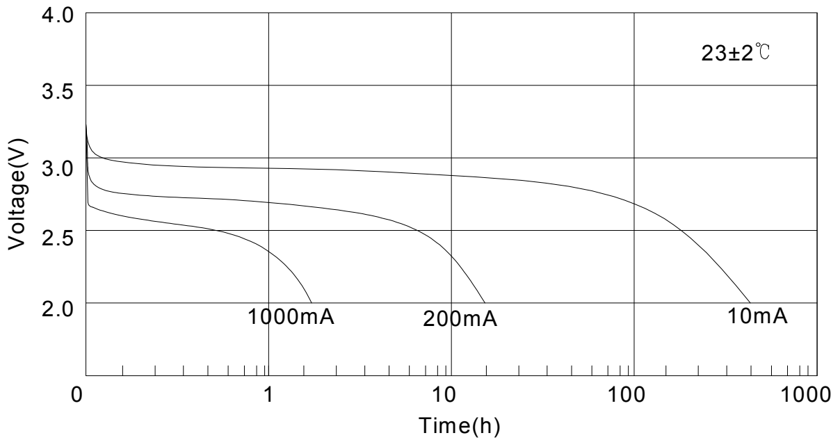
Discharge performance
