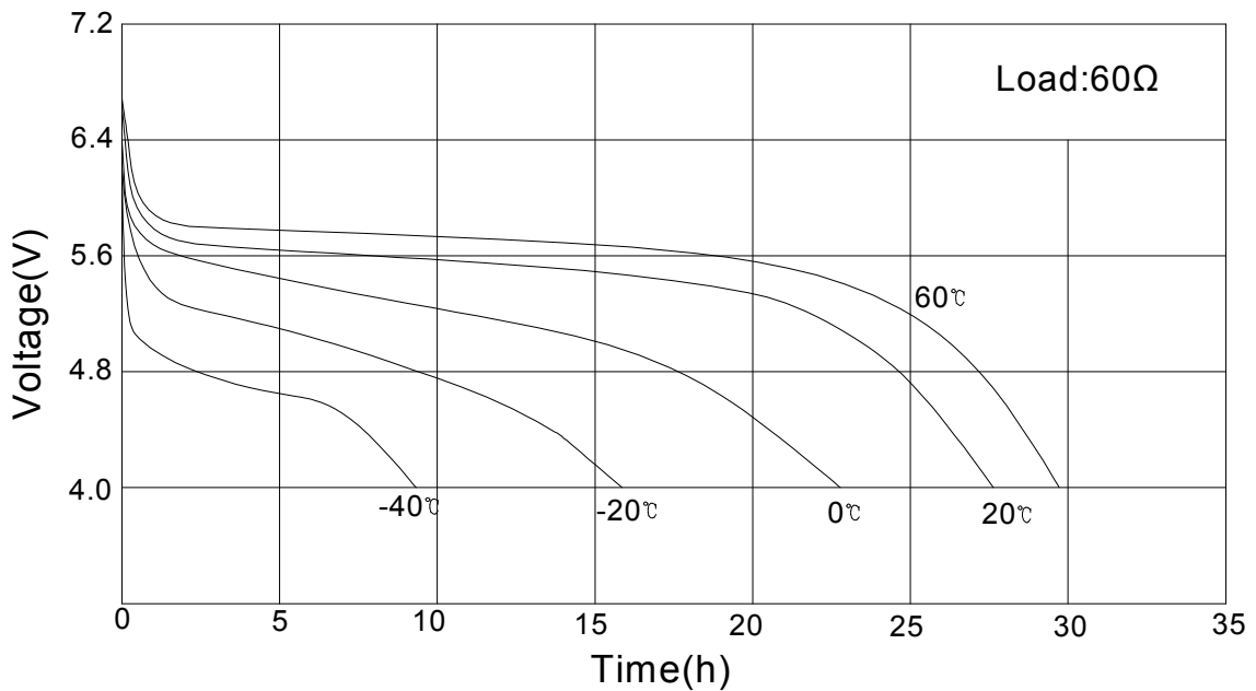
The relationship between Voltage and temperature
