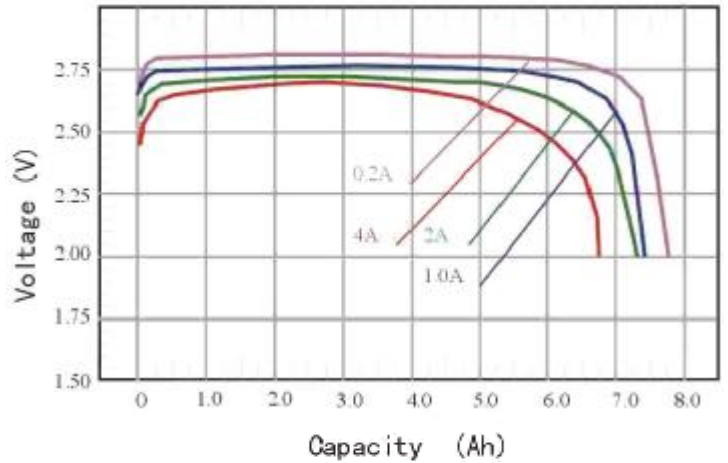
Discharge Characteristics at (20±2°C)
