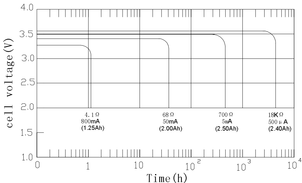
Discharge performance
