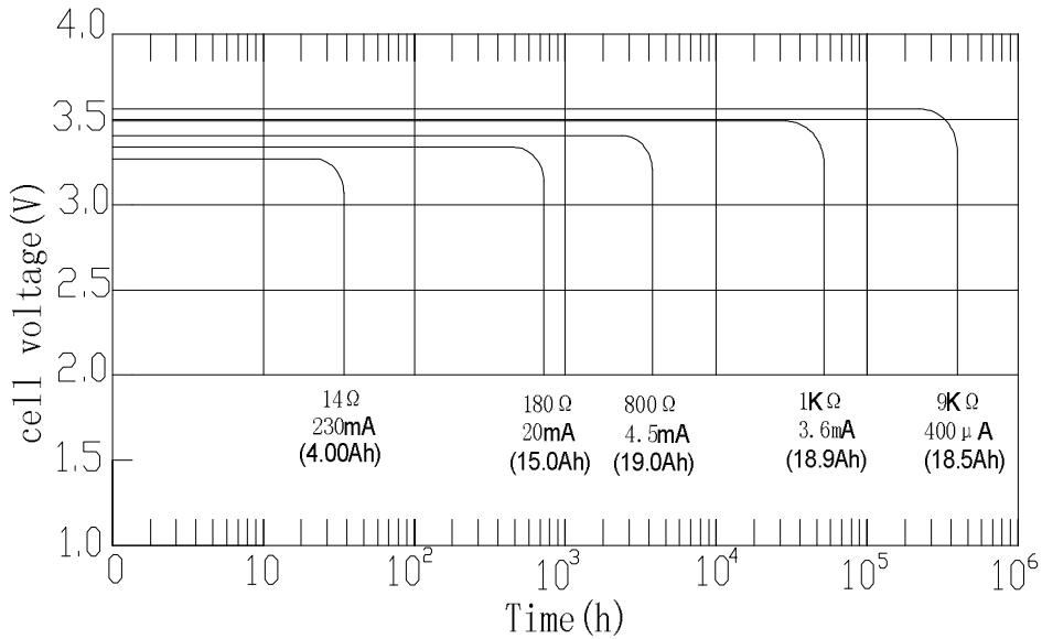
Discharge performance
