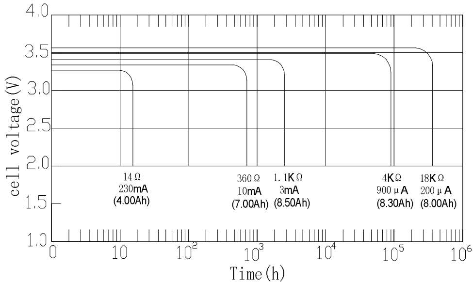
Discharge performance
