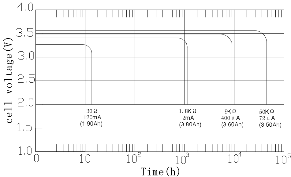
Discharge performance
