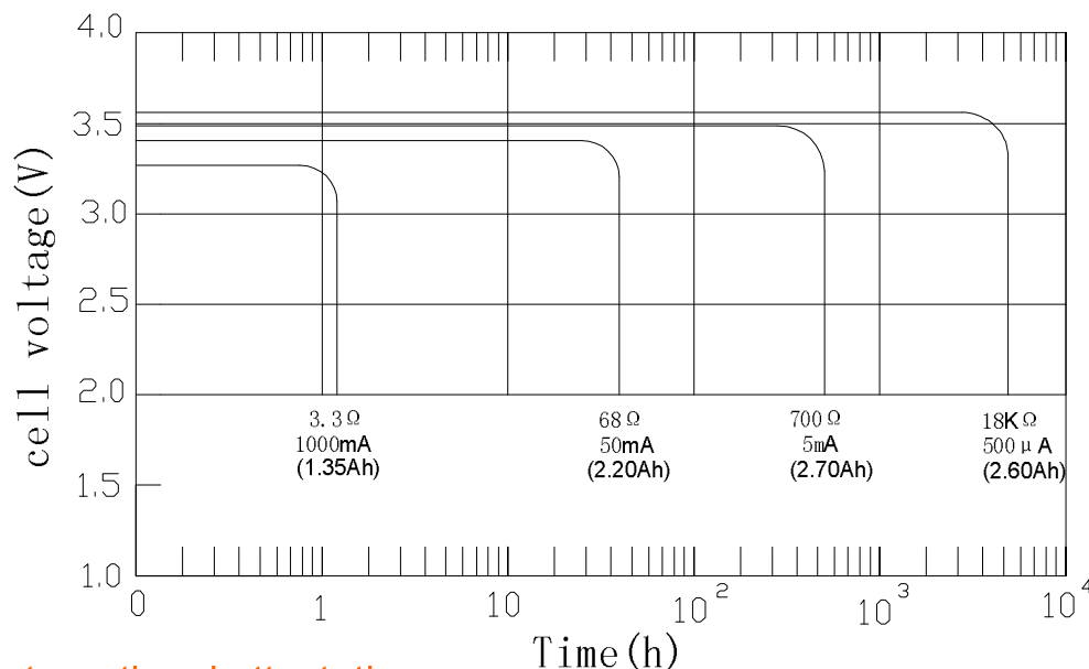
Discharge performance
